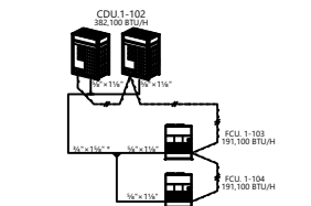
VRF AND CONTROL SCHEMATIC DIAGRAM 2/4
