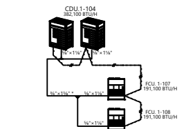
VRF AND CONTROL SCHEMATIC DIAGRAM 4/4
