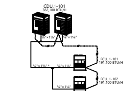
VRF AND CONTROL SCHEMATIC DIAGRAM 1/4
