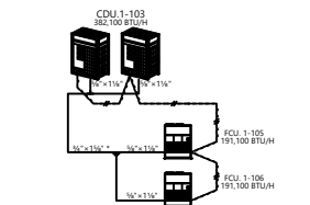
VRF AND CONTROL SCHEMATIC DIAGRAM 3/4
